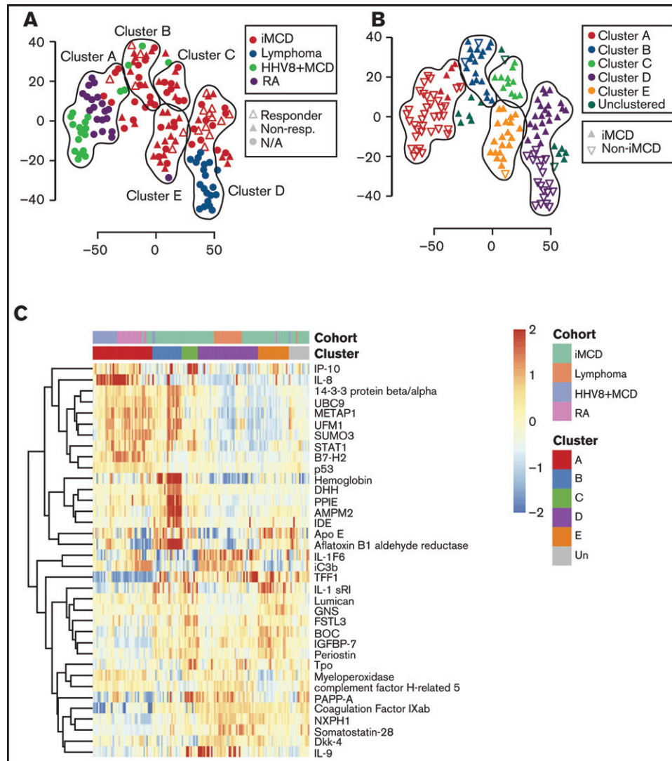
Figure 2. Clustering analysis of serum proteomes of iMCD and related diseases reveals notable heterogeneity. (A) A t -SNE plot visualizing serum proteomes of iMCD, Hodgkin lymphoma (lymphoma), HHV8-associated MCD (HHV8+MCD), and rheumatoid arthritis (RA) patients during active disease. Among the iMCD patients, siltuximab responders (partial response or complete response, per durable clinical and tumor [radiologic lymph node] response criteria as determined in NCT01024036) are indicated with open triangles, nonresponders with closed triangles, and patients for which siltuximab was not given as a monotherapy or response was not assessed by independent clinical trial review are represented by closed circles. Colored lines are drawn around clusters as determined by elastic net with fivefold cross-validation. (B) A revisualization of the t -SNE plot of iMCD and related disease serum proteomes to better indicate iMCD in relation to all other samples. Colored lines are drawn around clusters A to E as determined by elastic net with fivefold cross-validation, and samples within each cluster are colored accordingly. iMCD patients are indicated by a closed upward-facing triangle, and non-iMCD patients are visualized by an open downward-facing triangle. (C) Top 40 serum analytes that best distinguish between clusters A to E, as selected by elastic net with fivefold cross-validation, across iMCD and related disease samples.
